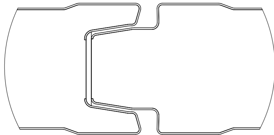
DETALLE JUNTA DEL PANEL / PANEL JOINT / JOINT DE PANNEAU ESCALA 1.5 : 1
