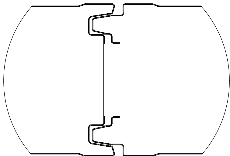
DETALLE JUNTA DEL PANEL / PANEL JOINT / JOINT DE PANNEAU ESCALA 1 : 1.5
