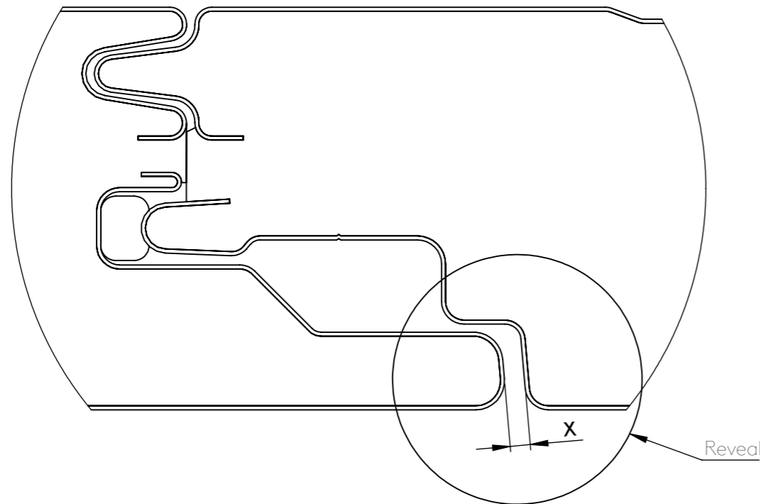
JUNTA DEL PANEL / PANEL JOINT / JOINT DE PANNEAU ESCALA 1.5 : 1
