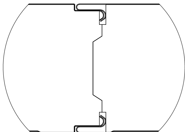
DETALLE JUNTA DEL PANEL / PANEL JOINT / JOINT DE PANNEAU ESPESORES ≥ 80mm
